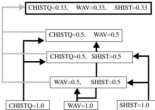
Fig. 3. Seven-subpopulation topology.
