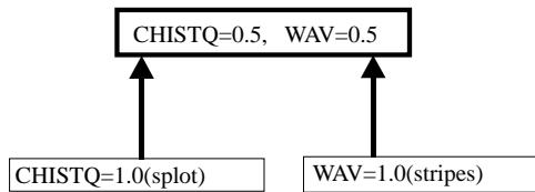
Fig. 4. Three-subpopulation topology.
