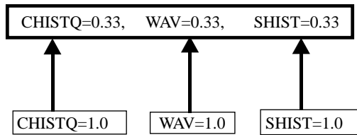
Fig. 2. Four-subpopulation topology.
