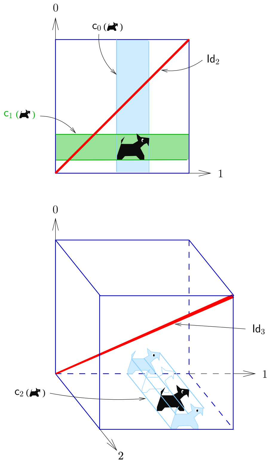
Fig. 1. Drawing cylindrifications in the case of n = 3 .
